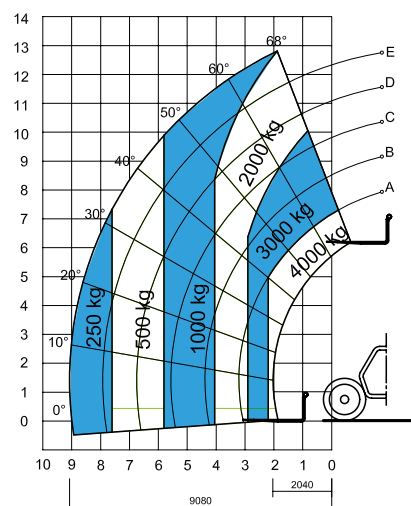
Lift capacity chart (without outriggers)****
