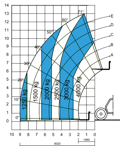
Lift capacity chart (with outriggers)****
